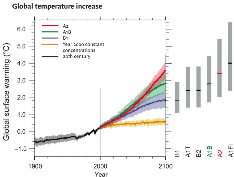
Figure 3. Model calculations of the global rise in temperature from 1900 to 2100 for three emission scenarios (see Box 3) as well as for the hypothetical situation where the atmospheric content of greenhouse gases remains constant at 2000 levels. All temperatures are shown relative to the mean temperature for 1980-1999 (Solomon et al. 2007).
